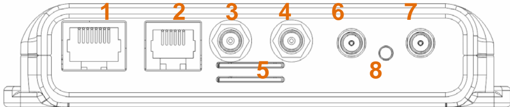
Figure 1. Front View (RL01w, RU01w)
