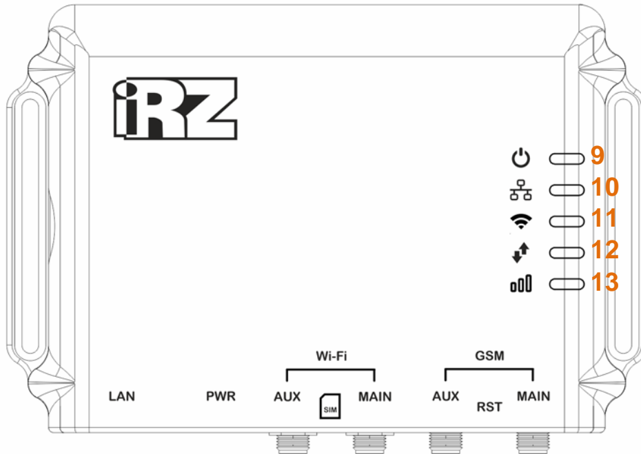
Figure 2. Top View
